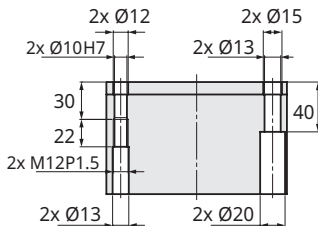
Detailed dimensions of dowel and mounting holes:
