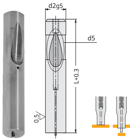
Code: BAFZ Heavy Duty Ball Lock Punch with Ejector (Blank type)
