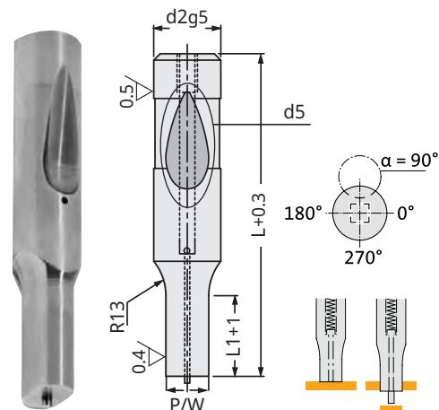
Code: BAF... Heavy Duty Ball Lock Stepped Punch with Ejector
