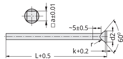
Conical Head Punch Shaped Code: HFY
