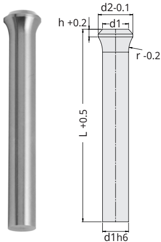
Bottle-neck Punch (Blank type) DIN 5118 (Trambone type)
