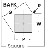
Code: BAF... Heavy Duty Ball Lock Stepped Punch with Ejector
