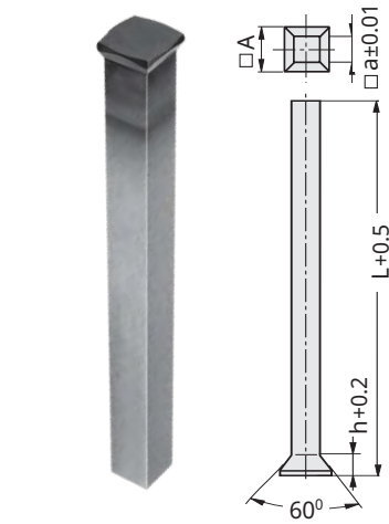
Slot - Form DA forged head Square Head Punch, Slot Stepped Code: HFK
